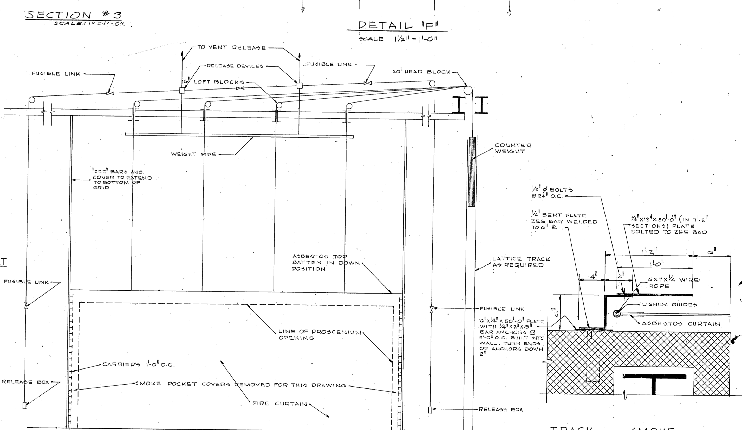
FIRE CURTAIN RIGGING AND ELEVATION DIVISION II
